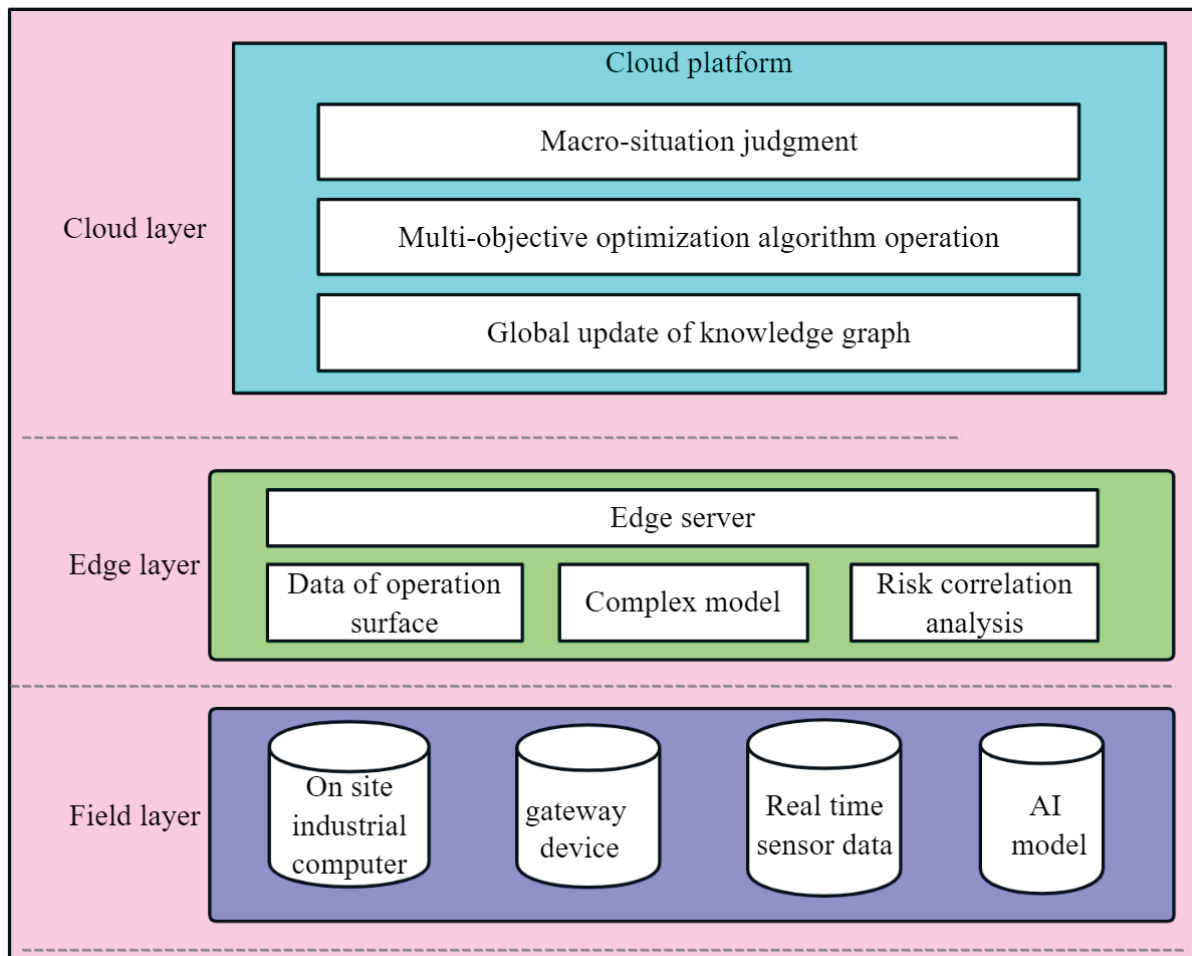
Figure 2 Intelligent decision-making and response architecture
